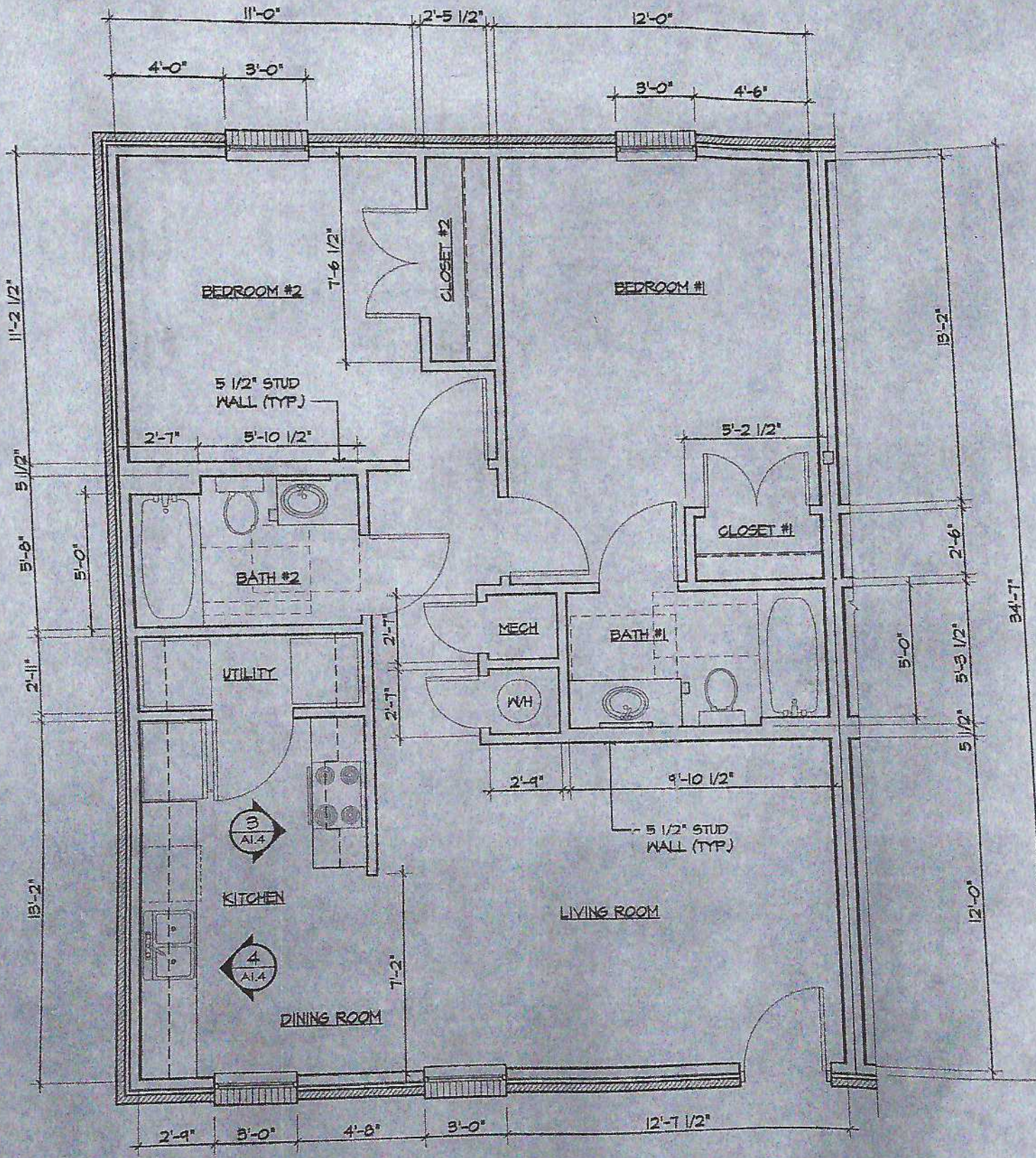
1 ENLARGED FIRST FLOOR ROOM PLAN (BUILDING A) 1/4" = 1'-0"
